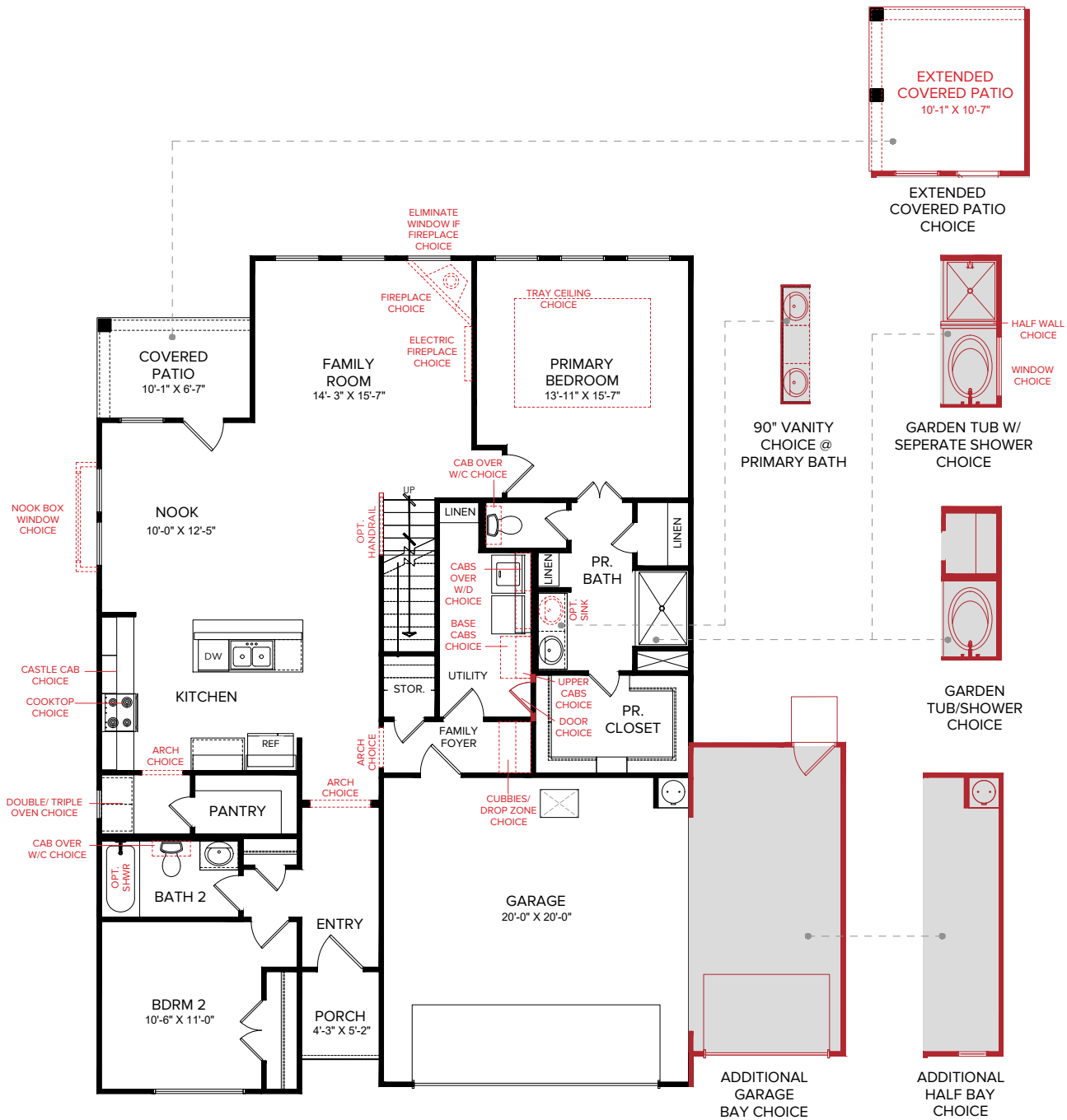
FIRST FLOOR
